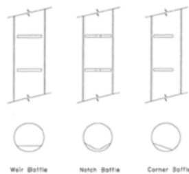
Figure 3. Different baffle designs (Environment Agency, 2010b).
